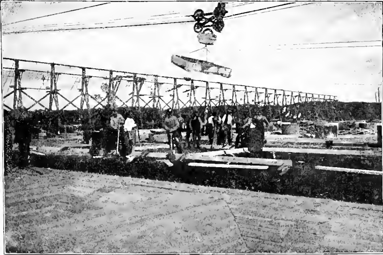
PLACING THE CONCRETE VAULTING.
